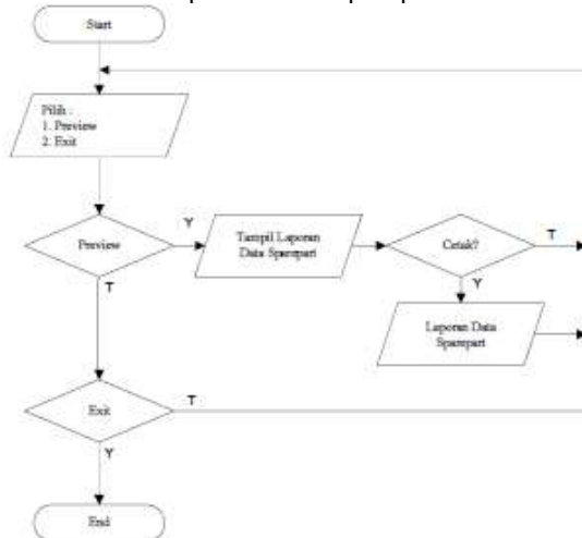
Gambar 12. Flowchart Laporan Data Sparepart
