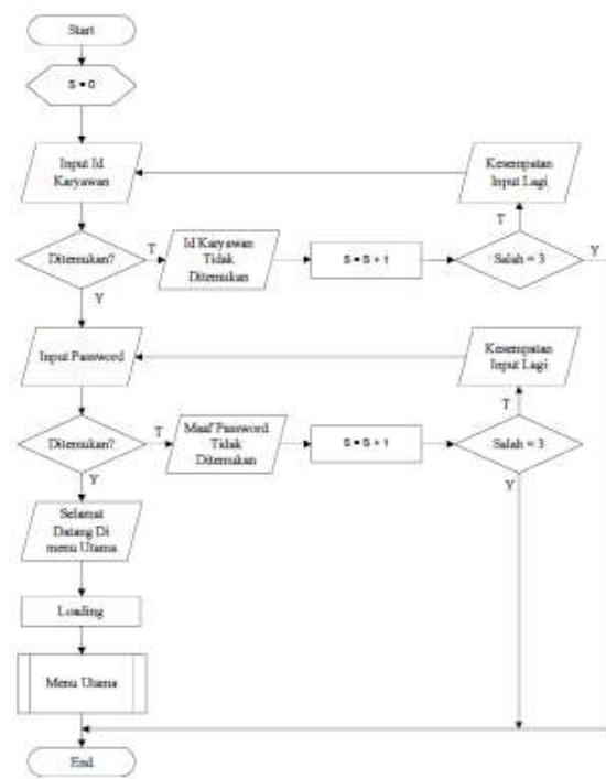
Gambar 6. Flowchart Program Login
